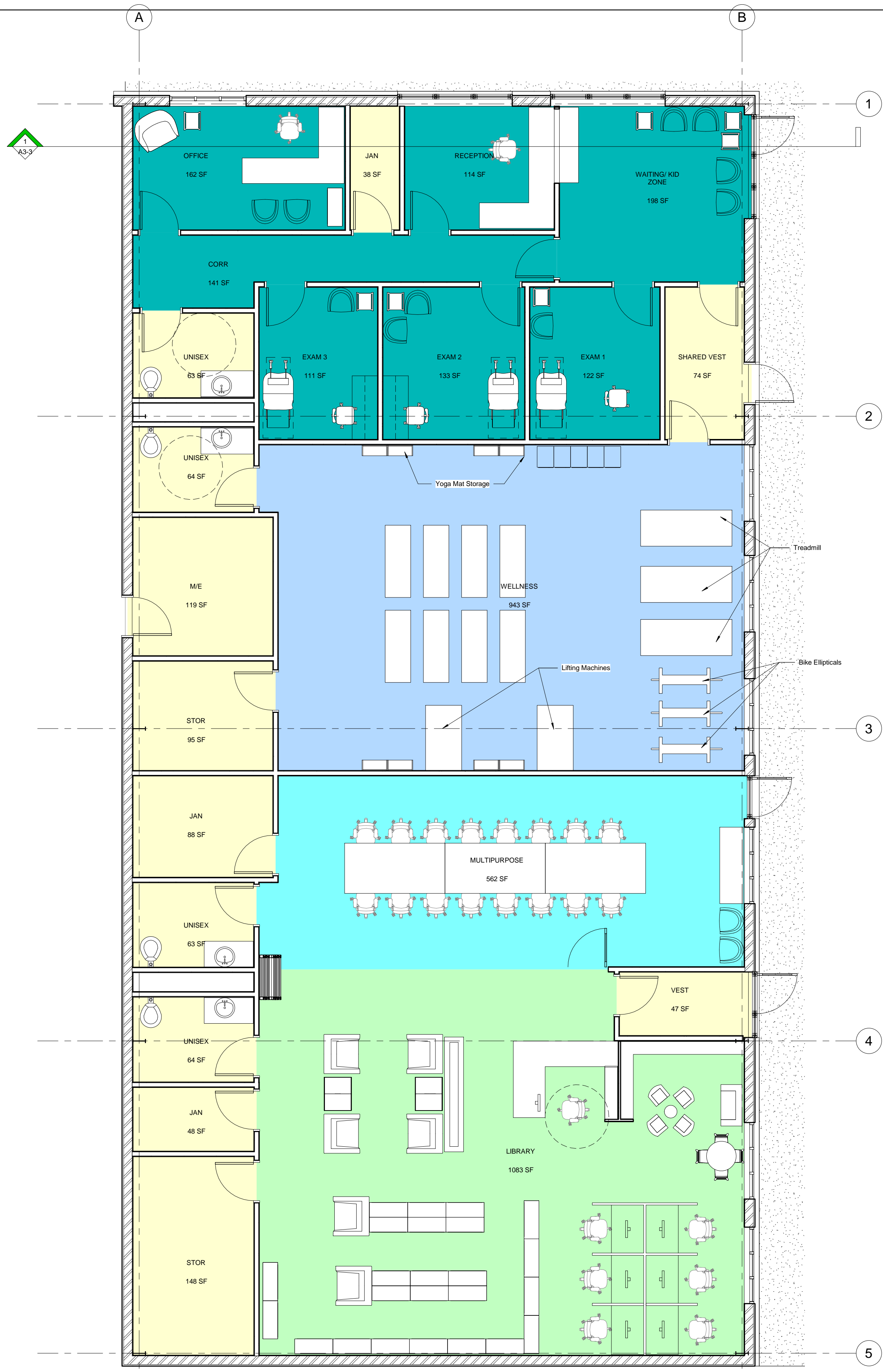
1 | LIBRARY AND WELLNESS CENTER- OPTION 2 SCALE: 1/4" = 1'-0"
